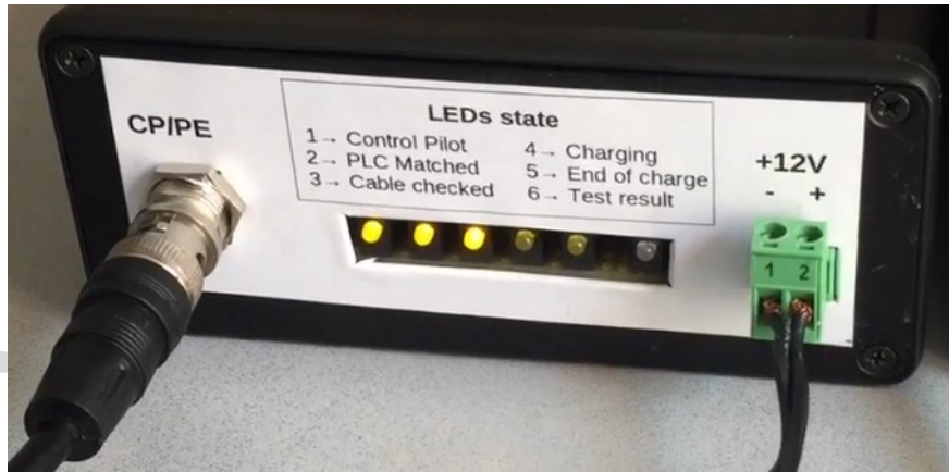
Figure 1: ComboCS4M showing charging session progress
